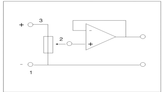
Recommended Measurement Circuit 用測試綫路
