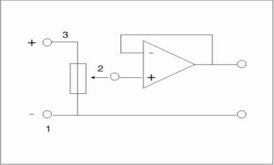
Recommended Measurement Circuit 用測試線路
